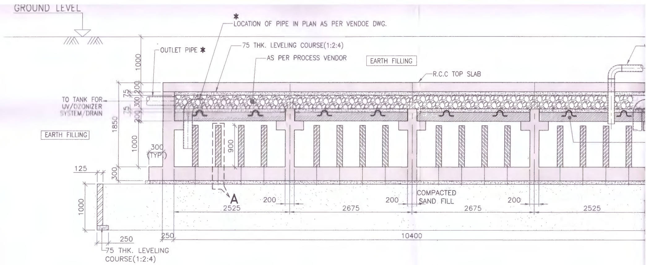
SECTION 2-2 (SCALE 1:50)
