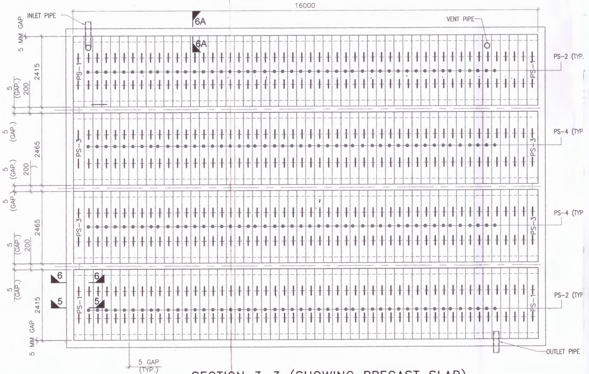
SECTION 3-3 (SHOWING PRECAST SLAB) (SCALE 1:75)
