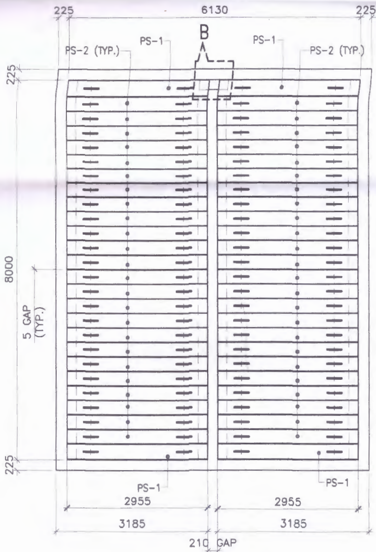
SECTION 4-4 (SCALE 1:75)
