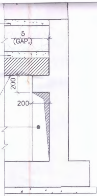
SECTION 6-6
