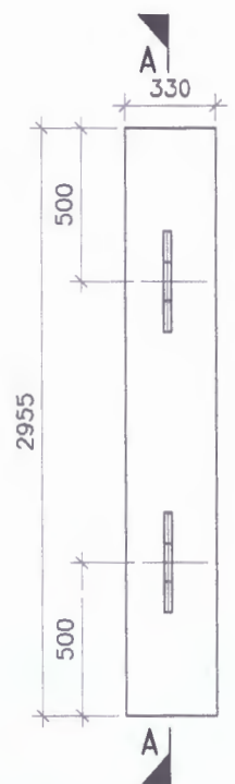
TYP. DETAIL OF PREC SLAB MKD. PS-1 (SCALE 1:25)
