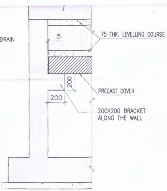
DETAIL - 5
