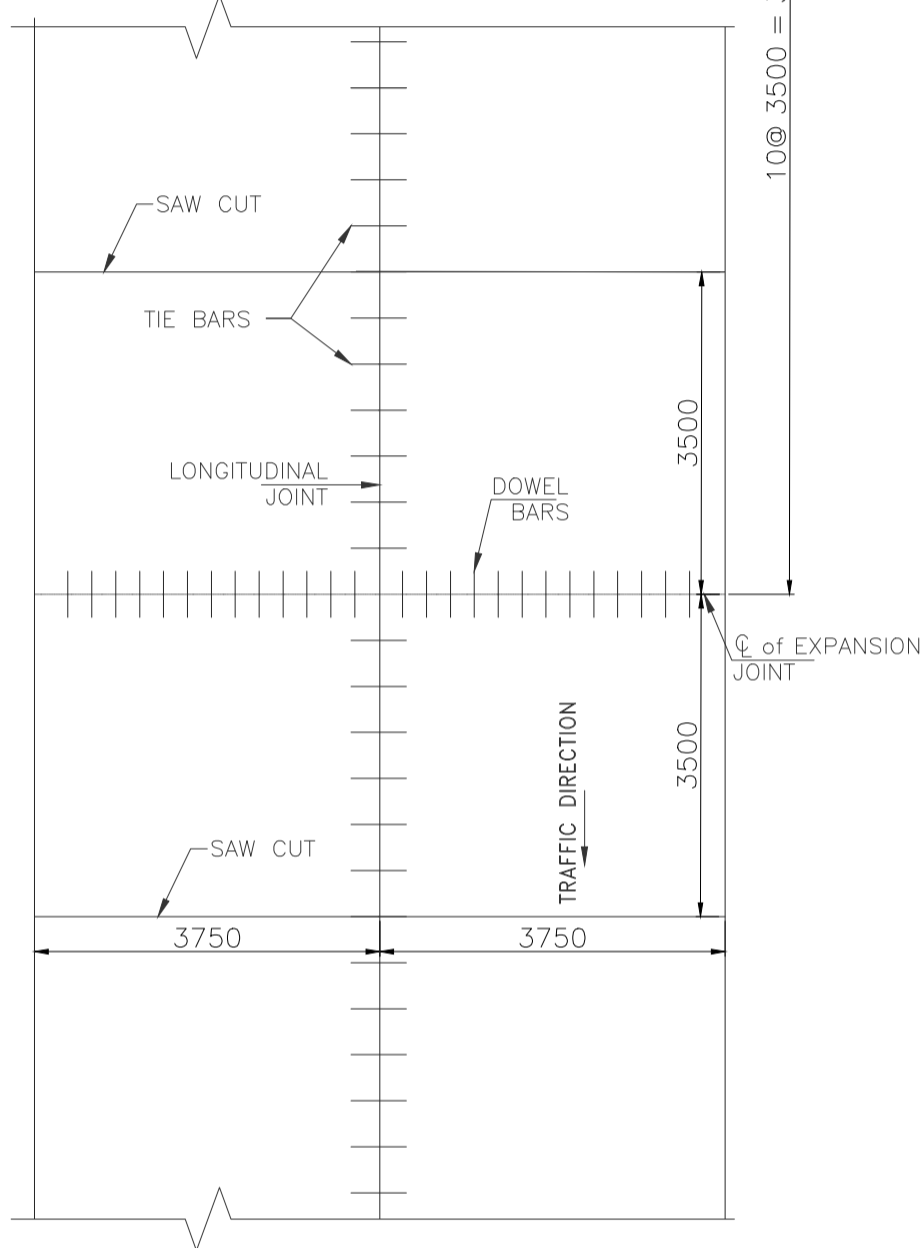
TYPICAL LAYOUT OF CONCRETE PANELS
