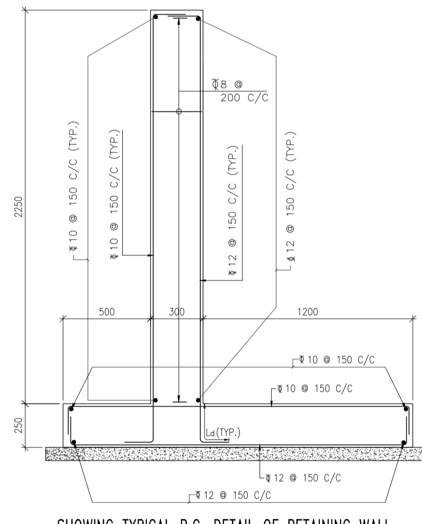
SHOWING TYPICAL R.C. DETAIL OF RETAINING WALL (SCALE-1:20)
