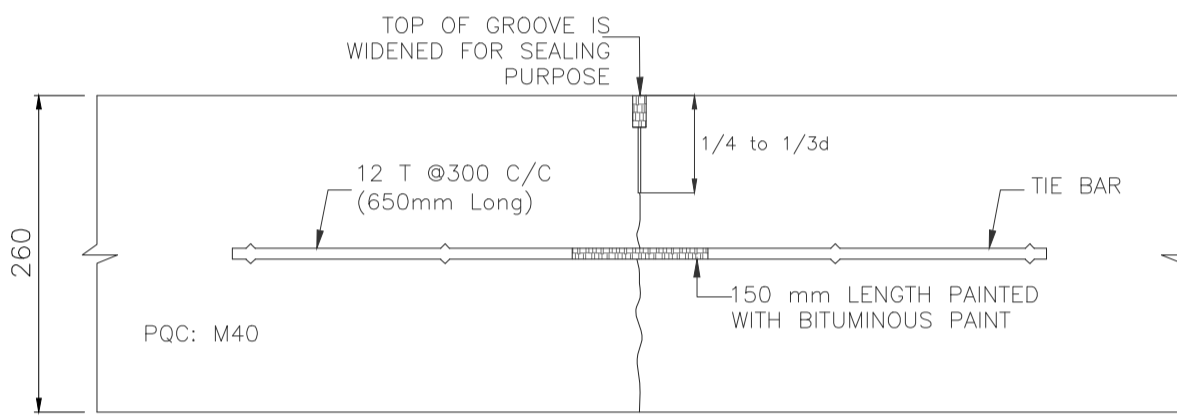
B: LONGITUDINAL JOINT WITH TIE - ROD BETWEEN TWO LANES
