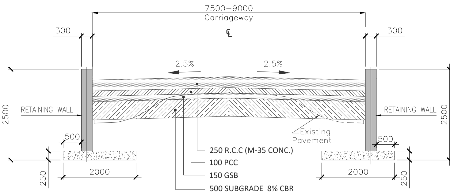
TYP. DETAIL OF ROAD WITH DRAIN
