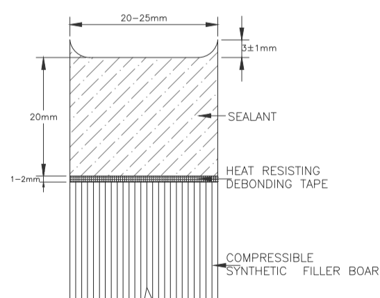
EXPANSION JOINT
