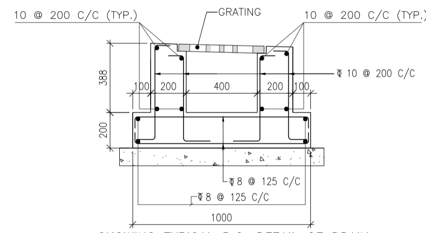
SHOWING TYPICAL R.C. DETAIL OF DRAIN (SCALE-1:20)
