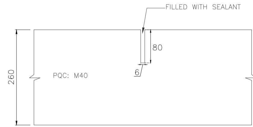
A: DETAILS OF SAW CUT
