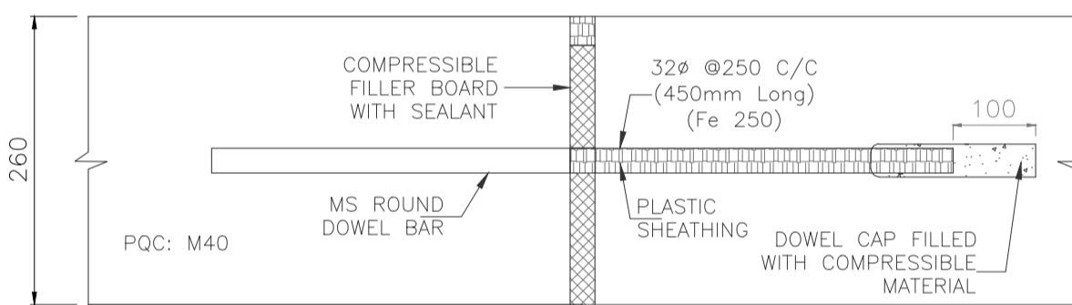
C: EXPANSION JOINT WITH DOWEL
